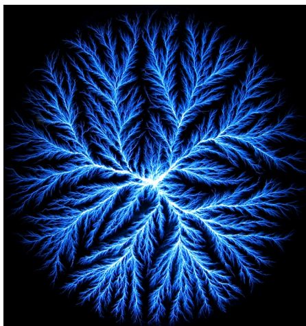
Lichtenberg "lightning", formed by rapidly discharging electrons in lucite. Scale = 10 cm = 10^{-1} m.
