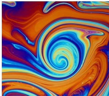
The turbulent motion of fluids creates spirals in systems ranging from a soap film to the oceans, atmosphere and the surface of Jupiter. Scale = 5 mm = 5 \times 10^{-3} m.
