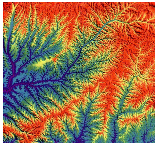
River network in China, formed by erosion from repeated rainfall flowing downhill for millions of years. Scale = 300 km = 3 \times 10^5 m.
