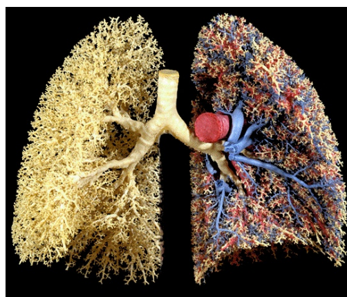
Our lungs are branching fractals with a surface area \sim 100 \text{ m}^2 . The similarity to a tree is significant, as lungs and trees both use their large surface areas to exchange oxygen and \text{CO}_2 . Scale = 30 cm = 3 \times 10^{-1} m.
