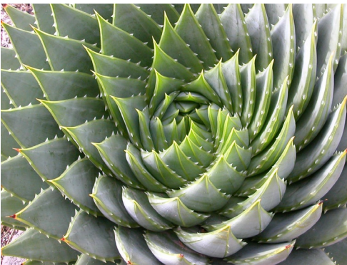
The plant kingdom is full of spirals. An agave cactus forms its spiral by growing new pieces rotated by a fixed angle. Many other plants form spirals in this way, including sunflowers, pinecones, etc. Scale = 50 cm = 5 \times 10^{-1} m.
